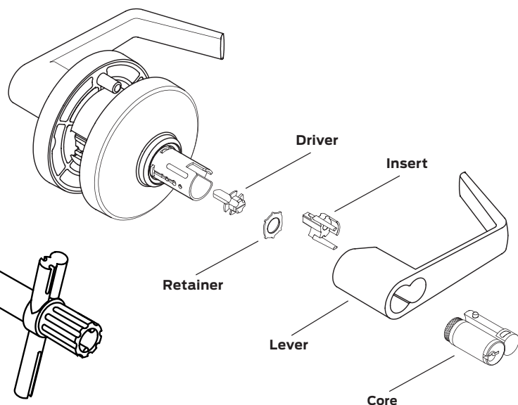
Full size IC conversion
